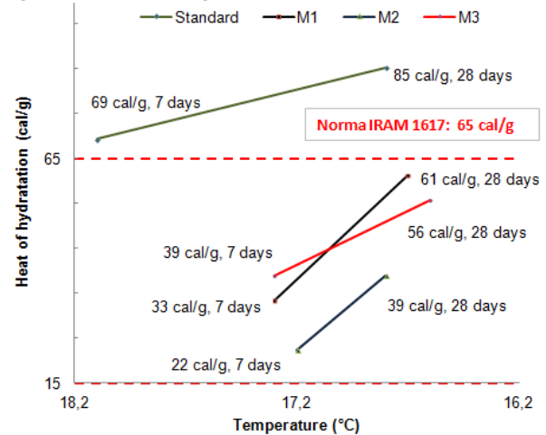
Figure 5: Hydration Heat.
