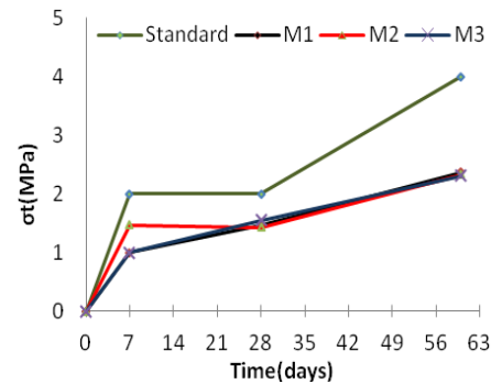
Figure 4: Tensile Strength Test.
