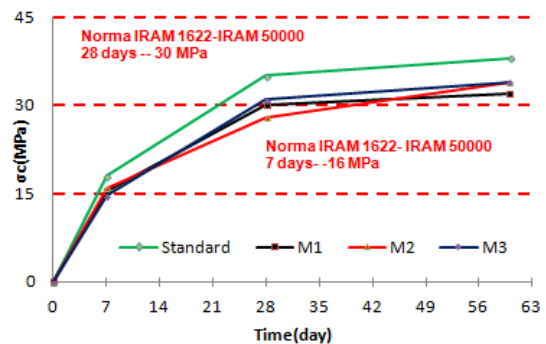
Figure 3: Compressive strength test.
