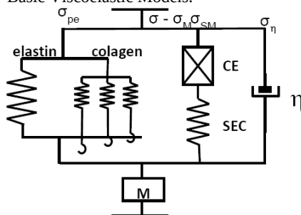
Figure 2. Modified Maxwell Model
