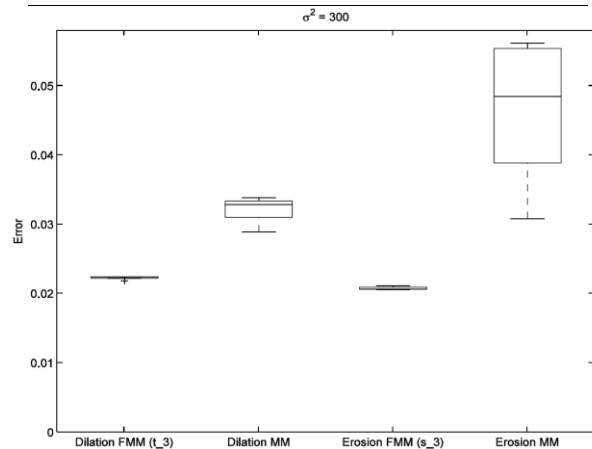
Figure 5: Box-plot of error rates comparing the classic mathematical morphology (MM) and the fuzzy morphology (FMM) based on the Bounded t-norm and s-conorm, for both dilation and erosion, and for the largest amount of noise ( \sigma^2=300 ), across all the structuring element sizes.
