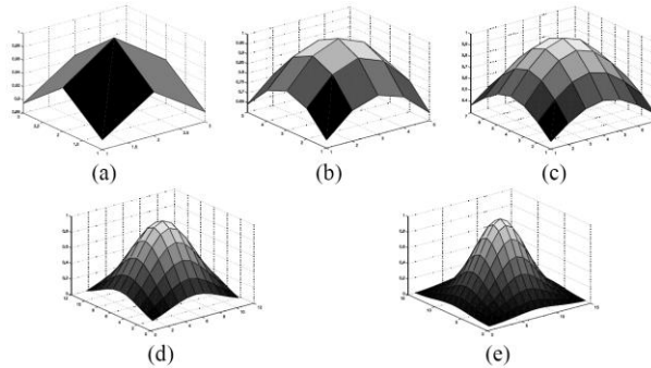
Figure 3: 3D view of the 5 structuring elements used for the FMM. (a) 3x3, (b) 5x5, (c) 7x7, (d) 11x11, (e) 15x15.
