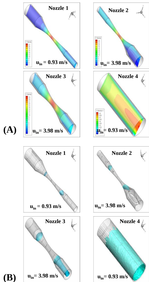
Fig. 2. (A) Velocity profile along the nozzles axis. (B) Flow pattern in each nozzle as the gas passes through. u_{in} is the inlet gas velocity.
