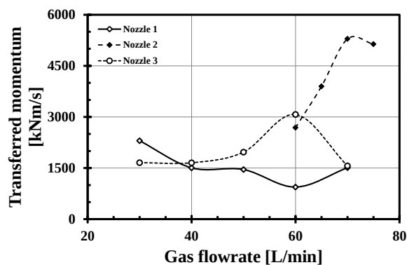
Fig. 6. Transferred momentum from the gas to the liquid using nozzles 1, 2, and 3.
