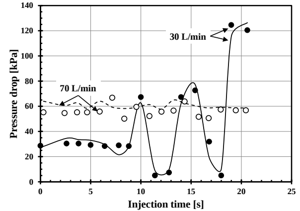
Fig. 5. Pressure drop comparison for gas injection using nozzle 1 at 30 and 70 L/min. (Points indicate experimental measurements, lines calculated values).
