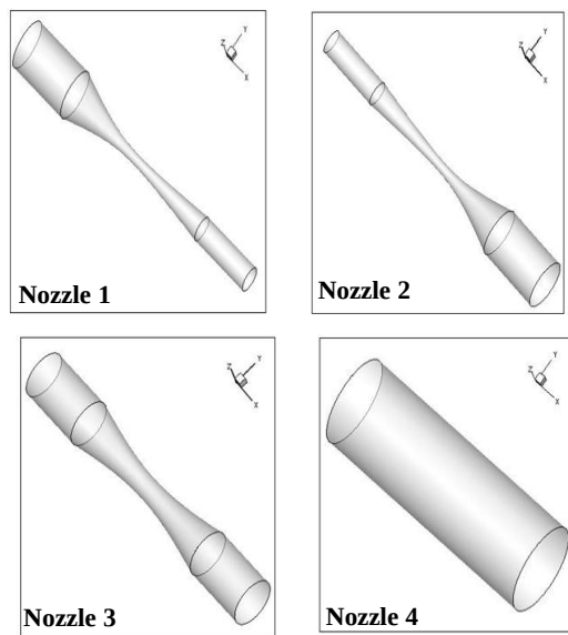
Fig. 1. (A) General description of a convergent-divergent nozzle. (B) Nozzles used for calculation.
