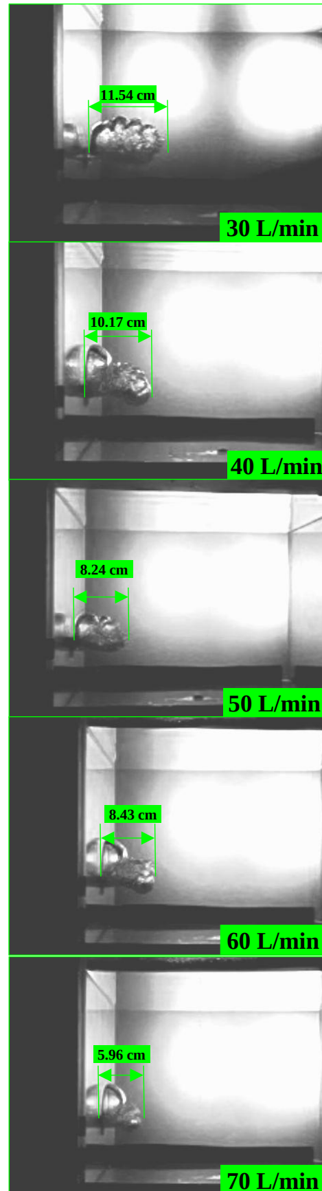
Fig. 7. Penetration of gas into the liquid pool as a function of the gas flowrate. In every case nozzle 1 was used to inject the gas.
