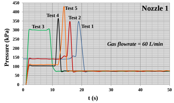
Fig. 4. Initial air injection in water at 60 L/min using nozzle 1.
