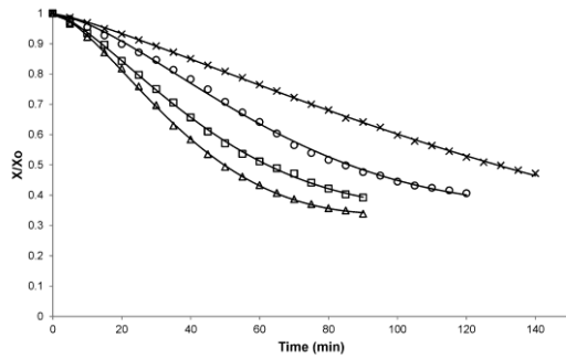
Fig. 1. Drying kinetics of mango peels at 100 (Δ), 80 (□), 60 (○) and 40 °C (x). Data presented, fitted to a modified Midilli's model, are average values from two independent experiments with standard errors less than 6%.
