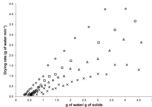
Fig. 2. Curves of drying rates versus moisture content during drying of mango peels at 100 (Δ), 80 (□), 60 (○) and 40 °C (x).
