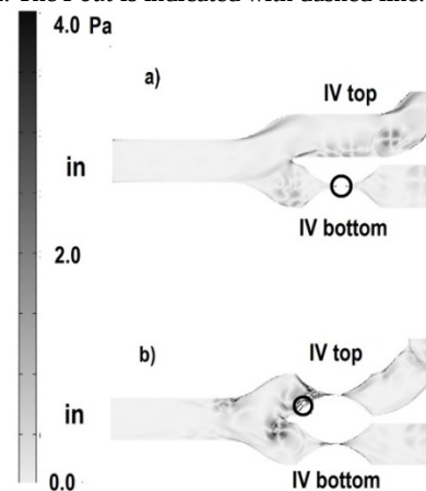
Figure 6. Representative shear stress at the input. In each figure the black circle indicates the maximum: a) \tau_{max} = 56 Pa at t = 476 ms and b) \tau_{max} = 65 Pa at t = 595 ms.
