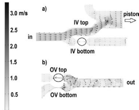
Figure 4. Velocity field: a) zoom of the input at 476 ms, with maximum v_p = 0.27 m/s; the black circle indicates the region where is the maximum fluid speed (1.71 m/s); b) zoom of the output at 595 ms, with v_p = -0.01 m/s; the black circle indicates the region where is the maximum fluid speed (3.28 m/s).
