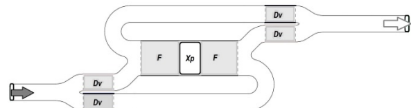
Figure 2. FEM mesh in different regions of the domain: mesh without deformation (in white), deformable mesh (in grey). Mesh regions in the chambers ( F ) are deformed according to the movement of the piston ( v_p ) and mesh regions in the valves are deformed accordingly their movements ( V_v ). The input and output sections are indicated with dark grey and white arrows respectively.
