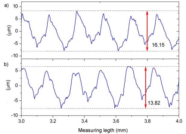
Fig. 3. Surface profiles of a ring with initial R_a = 2.85 \mu\text{m} : (a) before testing; (b) after testing.
