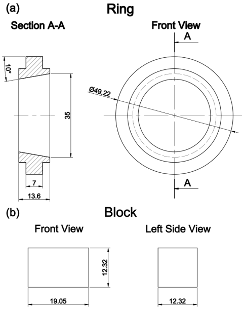
Fig. 2. Samples design and geometry.
