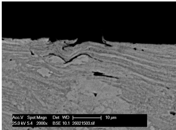
Fig. 9. Scanning electron microscope (SEM) micrograph in side view of the wear scar in a section normal to the sliding direction of a block specimen tested with R_a=1.27\ \mu\text{m} .
