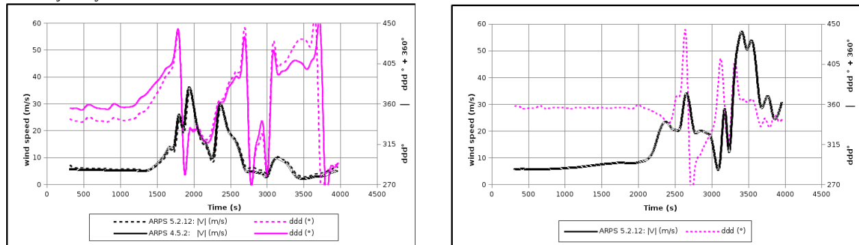
Figure 13: Temporal evolution of the wind speed simulation ( |V| m/s) and direction ( ddd^\circ ) at 22 meters over the ground in the place where the electrical transmission network pylons broke and fell.
