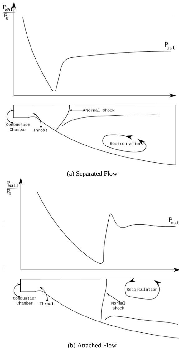
Figure 4: Schematic diagram of the flow transition during startup.
