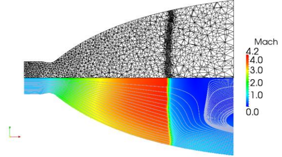
(a) Streamlines and Mach number distribution.
