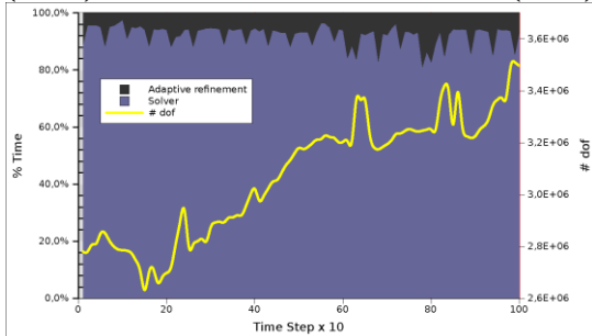
Figure 3: Relative cost of solver and adaptive refinement computations measured as clock time percentage during the simulation (number of degrees of freedom are shown on the right scale).
