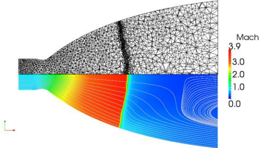
(a) Streamlines and Mach number distribution.
