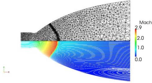
(a) Streamlines and Mach number distribution.
