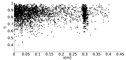
Figure 9: Mean-ratio shape measure along the axis of the nozzle for condition P_0 = 2.1 [MPa].
