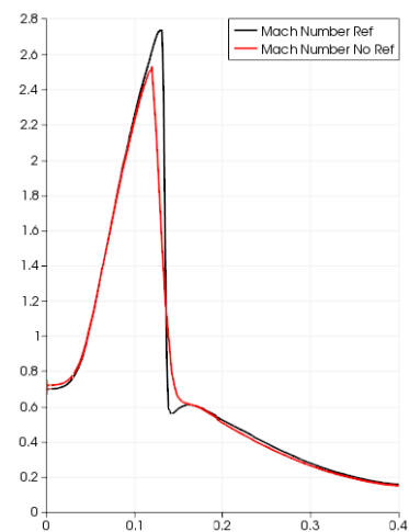
(b) Comparison of the Mach number distribution along the axis of the nozzle.
