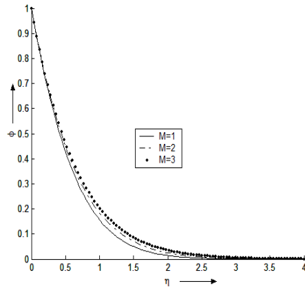
Figure 1. The graph of \phi against \eta , G_r=1 , Re=3 , G_c=3 , Pr=0.71 , S=0.2 , Br=2 , S_c=0.62 , \gamma=1 and t_d=0.001 for various values of M .
