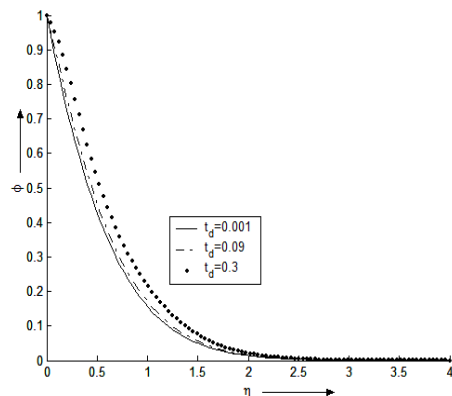
Figure 8. The graph of \phi against \eta , M=1 , G_r=1 , Re=3 , G_c=3 , Pr=0.71 , S=0.2 , Br=2 , S_c=0.62 and \gamma=1 for various values of t_d .
