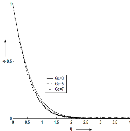
Figure 3. The graph of \phi against \eta , G_r=1 , Re=3 , M=1 , Pr=0.71 , S=0.2 , Br=2 , S_c=0.62 , \gamma=1 and t_d=0.001 for various values of G_c .
