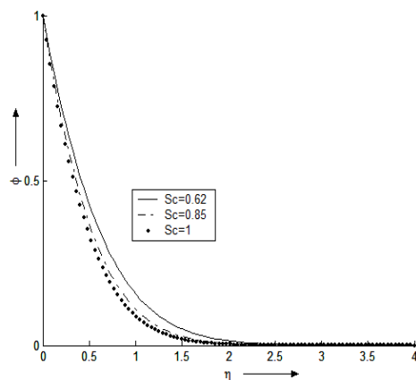
Figure 7. The graph of \phi against \eta , M=1 , G_r=1 , Re=3 , G_c=3 , Pr=0.71 , S=0.2 , Br=2 , \gamma=1 and t_d=0.001 for various values of S_c .
