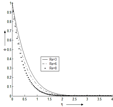
Figure 4. The graph of \phi against \eta , M=1 , G_r=1 , G_c=3 , Pr=0.71 , S=0.2 , Br=2 , S_c=0.62 , \gamma=1 and t_d=0.001 for various values of Re .
