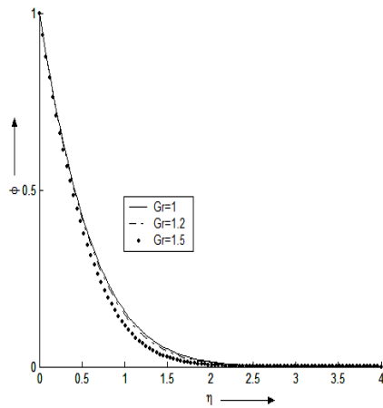
Figure 2. The graph of \phi against \eta , M=1 , Re=3 , G_c=3 , Pr=0.71 , S=0.2 , Br=2 , S_c=0.62 , \gamma=1 and t_d=0.001 for various values of G_r .
