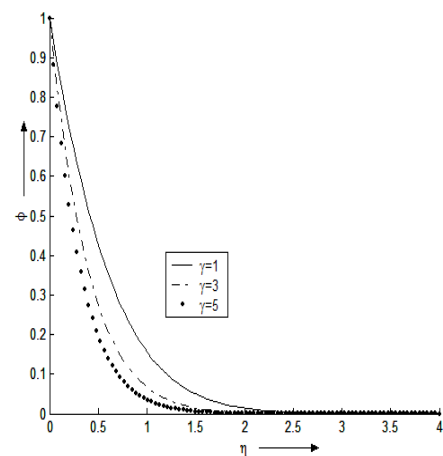
Figure 6. The graph of \phi against \eta , M=1 , G_r=1 , Re=3 , G_c=3 , Pr=0.71 , S=0.2 , Br=2 , S_c=0.62 and t_d=0.001 for various values of \gamma .
