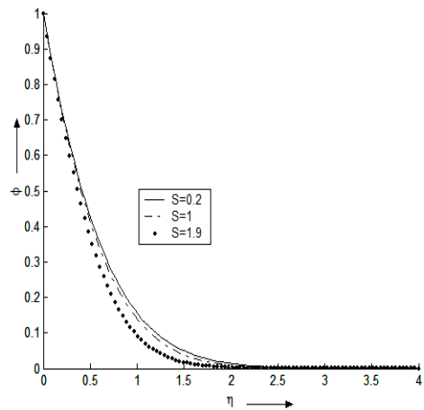
Figure 5. The graph of \phi against \eta , G_r=1 , Re=3 , G_c=3 , Pr=0.71 , M=1 , Br=2 , S_c=0.62 , \gamma=1 and t_d=0.001 for various values of S .
