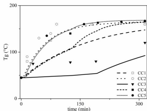
Fig. 5: Experimental data (in symbols) and theoretical results (in lines) for T_g as a function of time.
